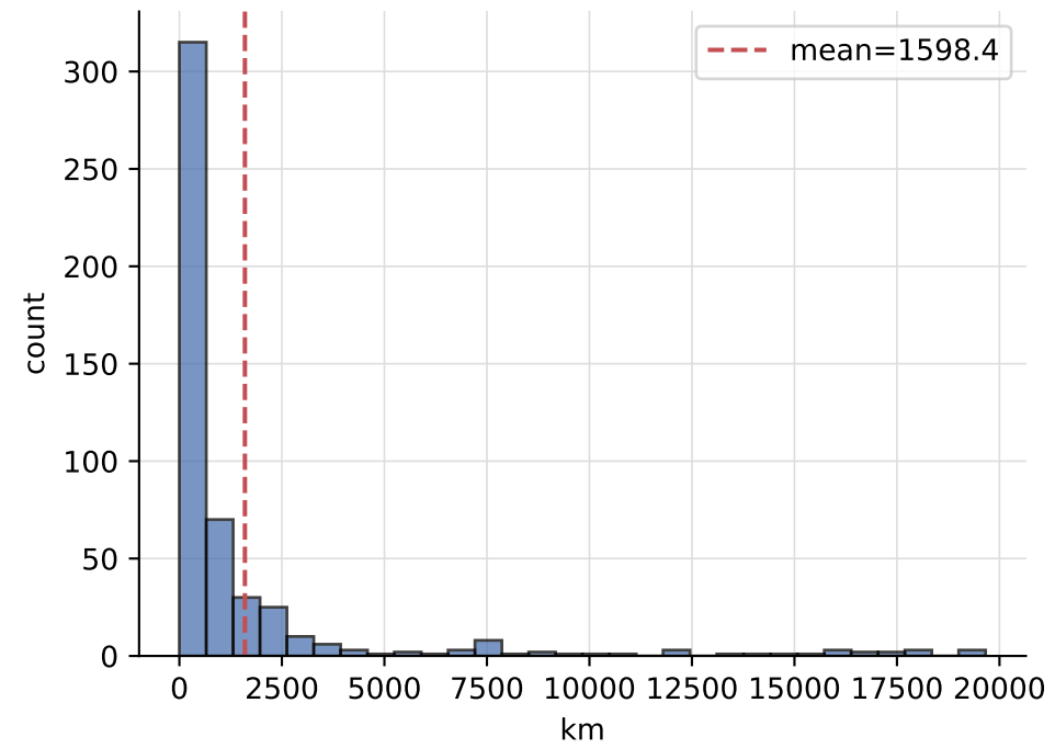
Haversine distance
